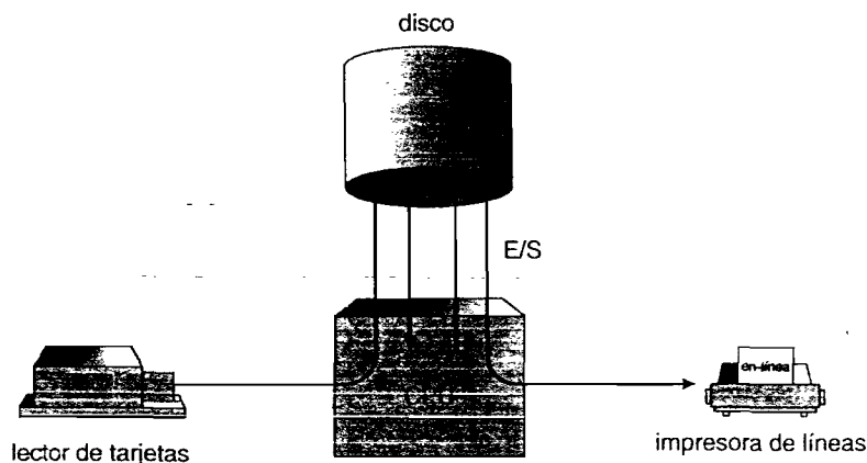
Figura 23.4 Spooling.
