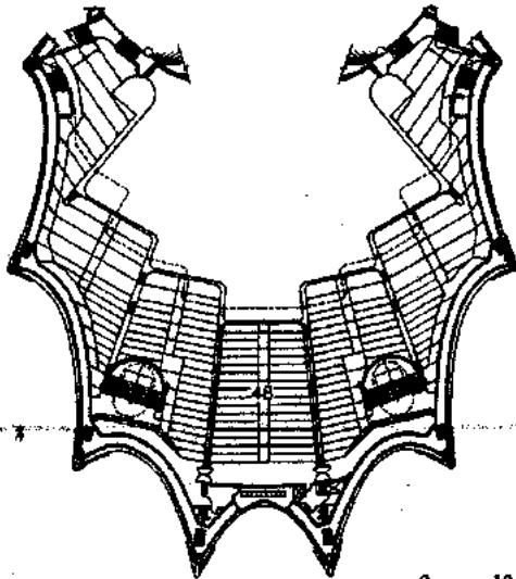
Planta mezzanine 1
