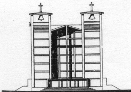
Fachada principal
