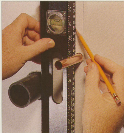
The supply pipes and drain of a kitchen sink are marked on the wall with the aid of a carpenter's level (above). The precise location of the fixtures will then be marked onto vertical and horizontal site story poles before being transferred to the story poles for the sink cabinet itself.
