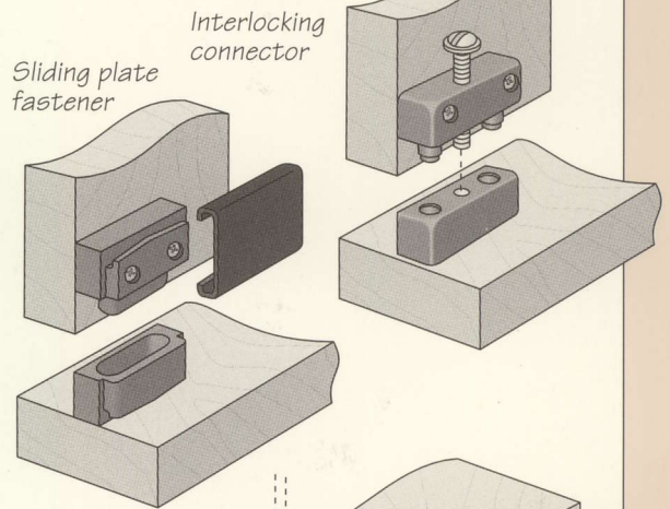
Pin joint connector
